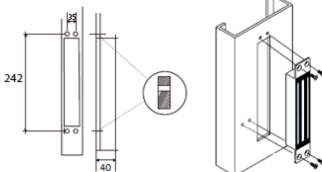
Electromagnet Fixation
