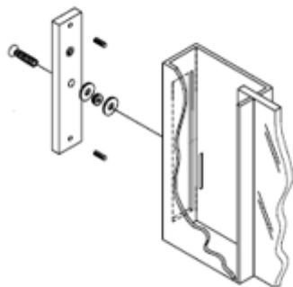
Plate Fixation
