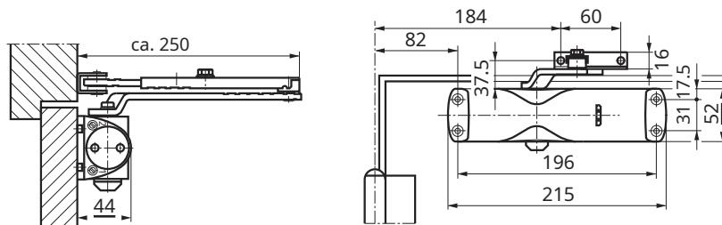
Measurements EN size 4, max. opening angle approx. 110°
