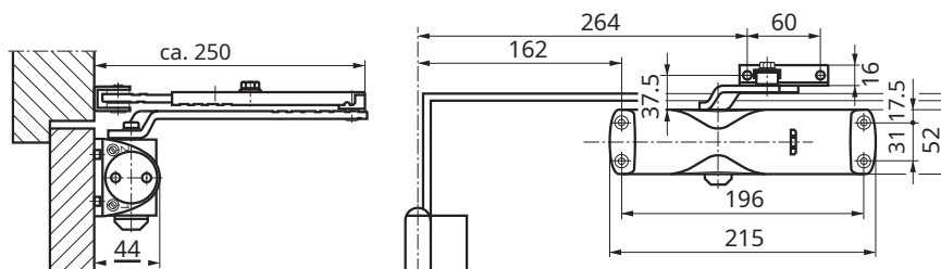
Measurements EN size 4, max. opening angle approx. 110°
