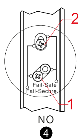
Fail Secure
