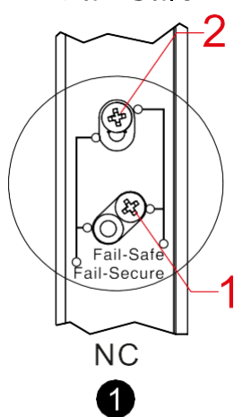
Fail-Safe
