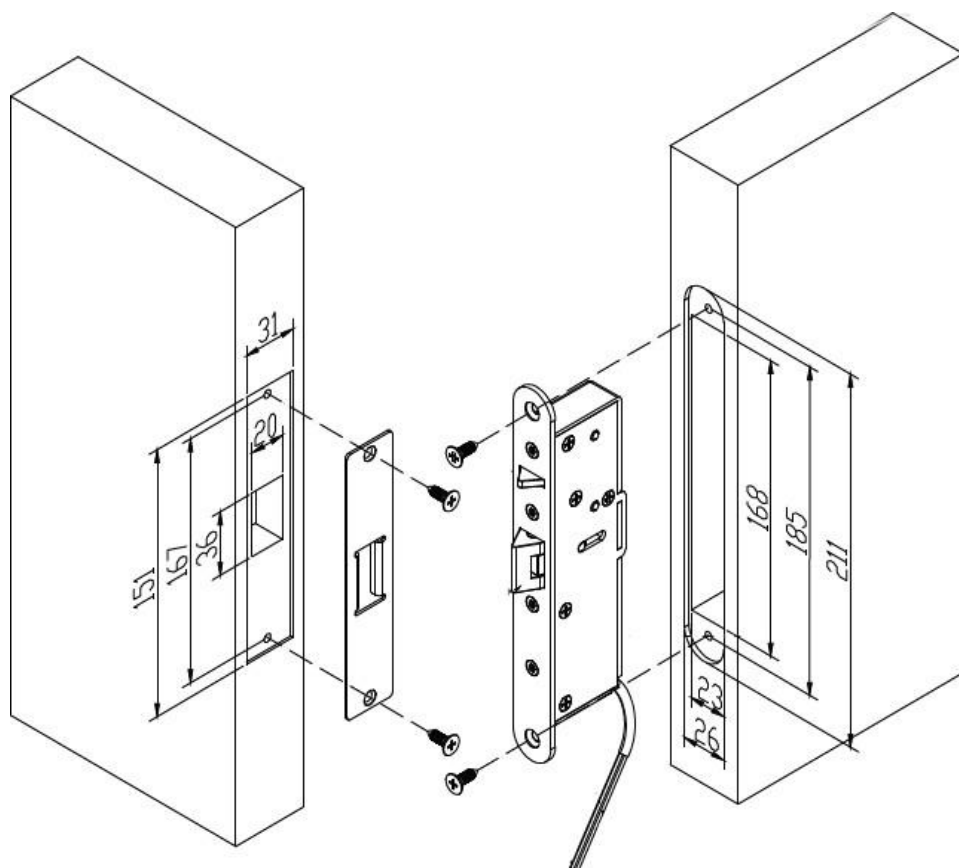
Fail-Safe
